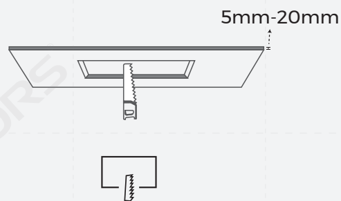
Opening size: 50x50mm
